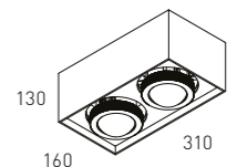
ZZOOM BASIC DOUBLE SURFACE - REFLECTOR
