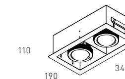
ZZOOM PULL-OUT DOUBLE RECESSED WITH TRIM
